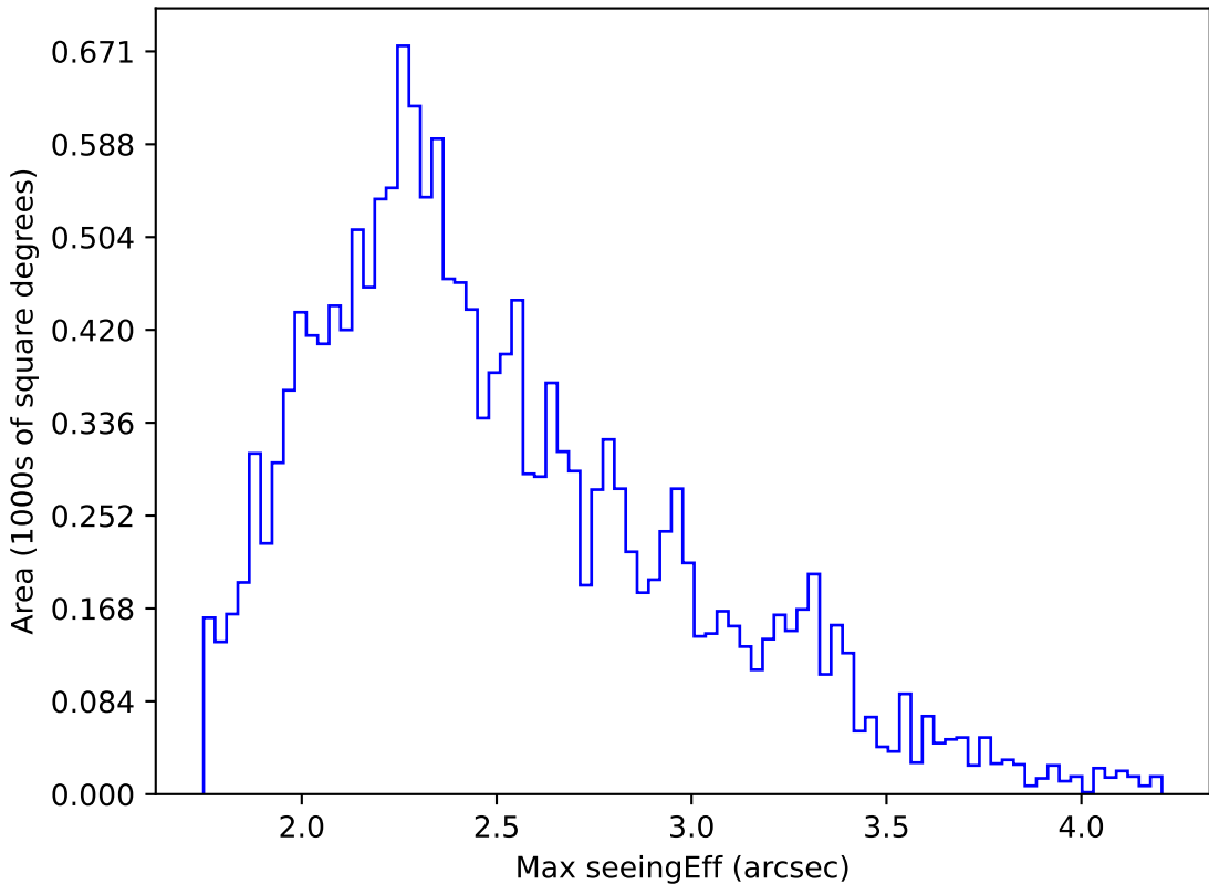
too_elab_r64_d2_ugrizy_v3.4_10yrs WFD u band: Max seeingEff
