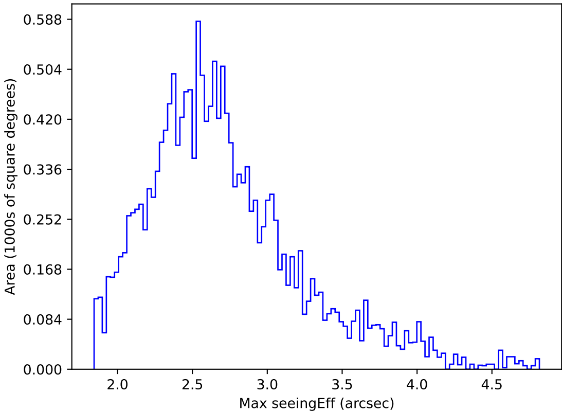
too_elab_r64_d2_ugrizy_v3.4_10yrs WFD r band: Max seeingEff
