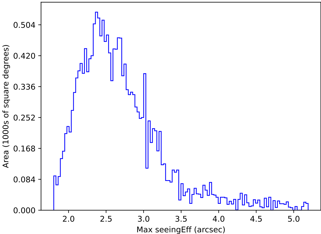
too_elab_r64_d2_ugrizy_v3.4_10yrs WFD i band: Max seeingEff
