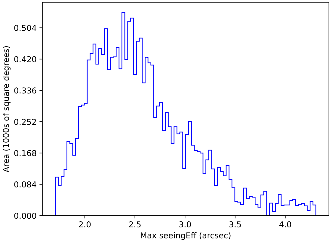
too_elab_r64_d2_ugrizy_v3.4_10yrs WFD g band: Max seeingEff
