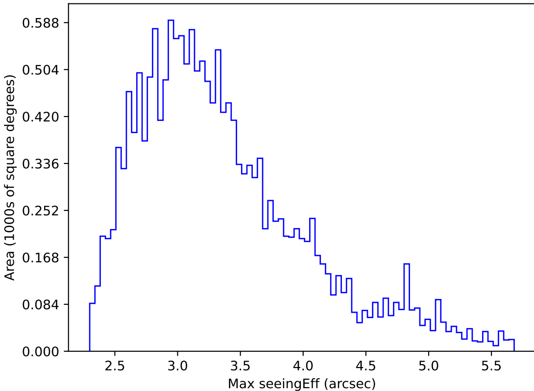
too_elab_r64_d2_ugrizy_v3.4_10yrs WFD all bands: Max seeingEff
