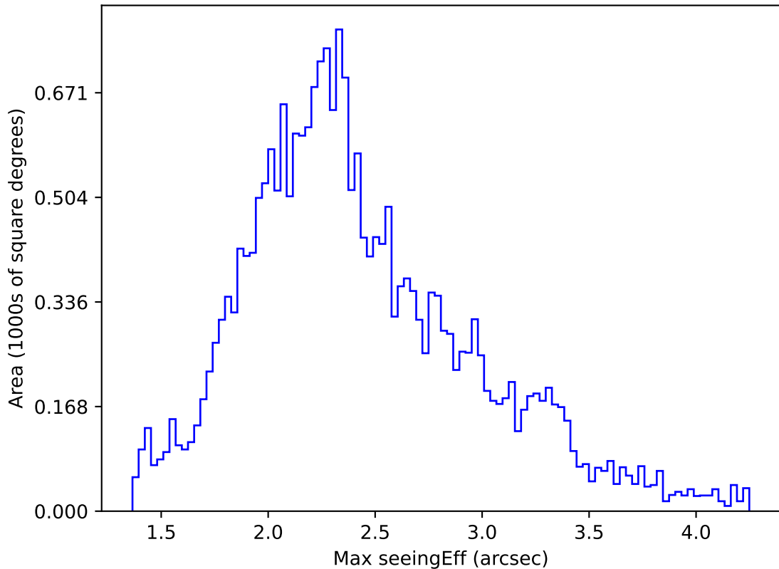
too_elab_r64_d2_ugrizy_v3.4_10yrs All sky u band: Max seeingEff
