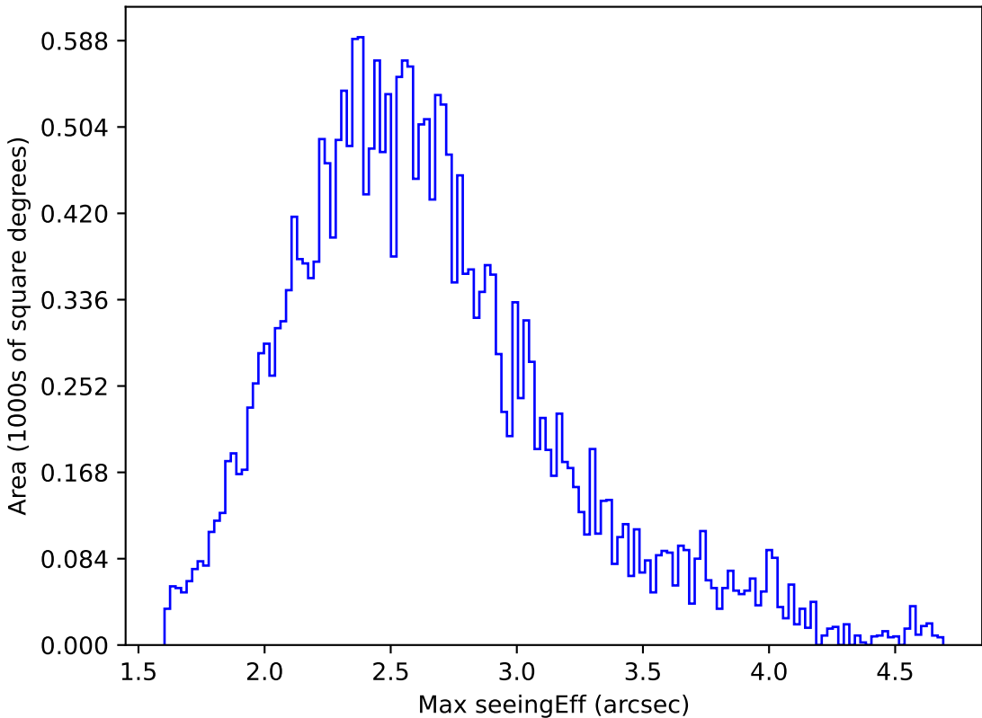
too_elab_r64_d2_ugrizy_v3.4_10yrs All sky r band: Max seeingEff
