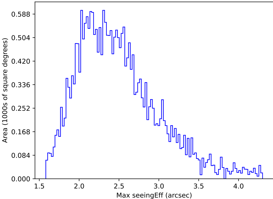
too_elab_r64_d2_ugrizy_v3.4_10yrs All sky g band: Max seeingEff
