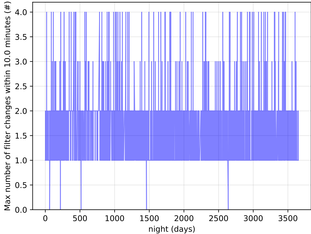
too_elab_r64_d2_ugrizyv3.4_10yrs Per Night: Max number of filter changes within 10.0 minutes
