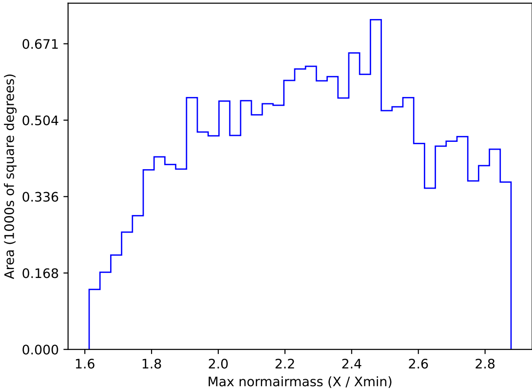
too_elab_r64_d2_ugrizy_v3.4_10yrs WFD z band: Max normairmass
