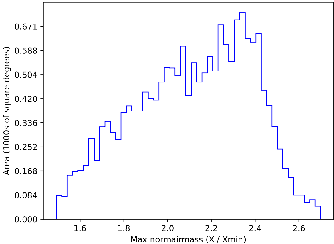
too_elab_r64_d2_ugrizy_v3.4_10yrs WFD r band: Max normairmass
