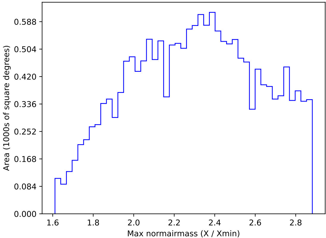
too_elab_r64_d2_ugrizy_v3.4_10yrs WFD i band: Max normairmass
