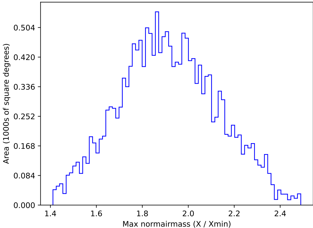
too_elab_r64_d2_ugrizy_v3.4_10yrs WFD g band: Max normairmass
