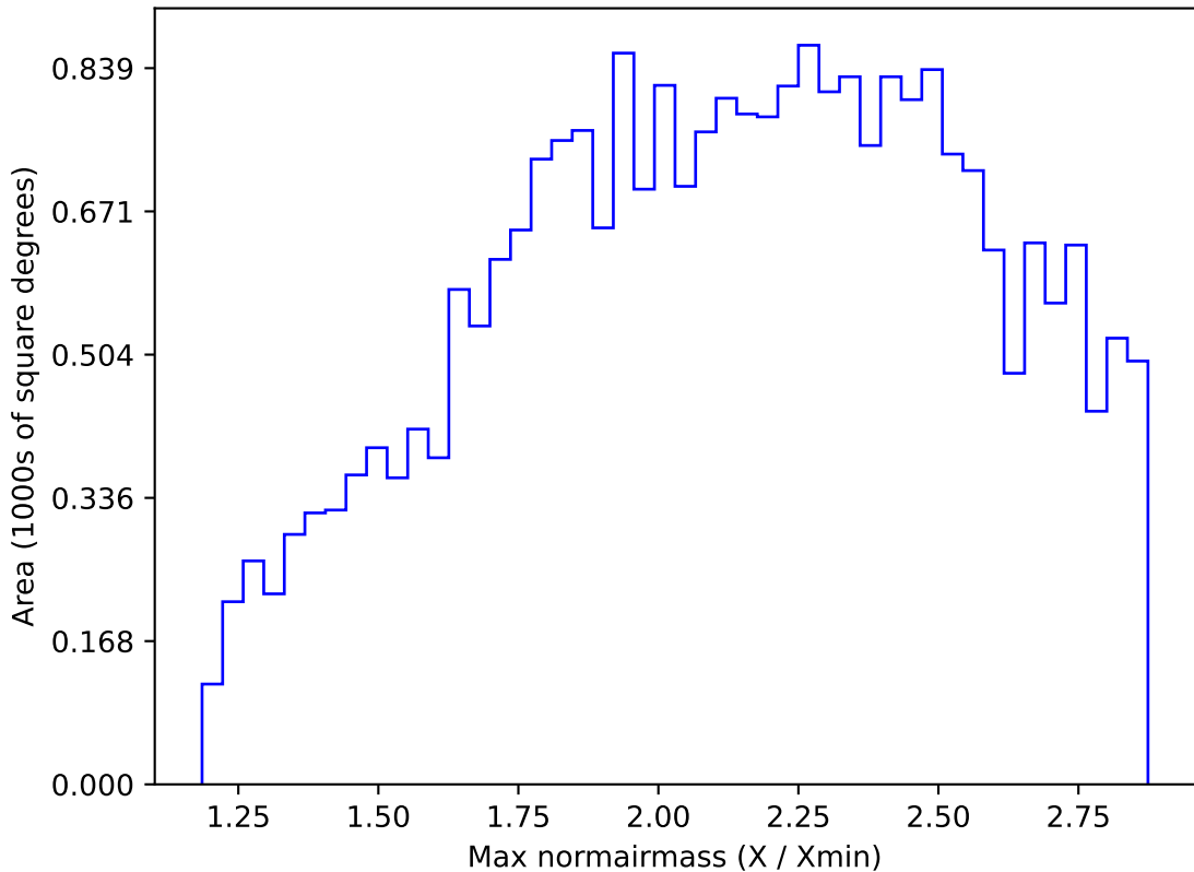
too_elab_r64_d2_ugrizy_v3.4_10yrs All sky z band: Max normairmass
