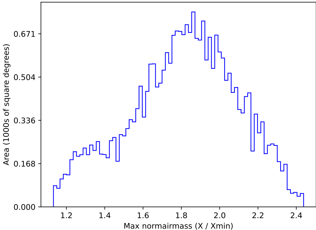
too_elab_r64_d2_ugrizy_v3.4_10yrs All sky g band: Max normairmass
