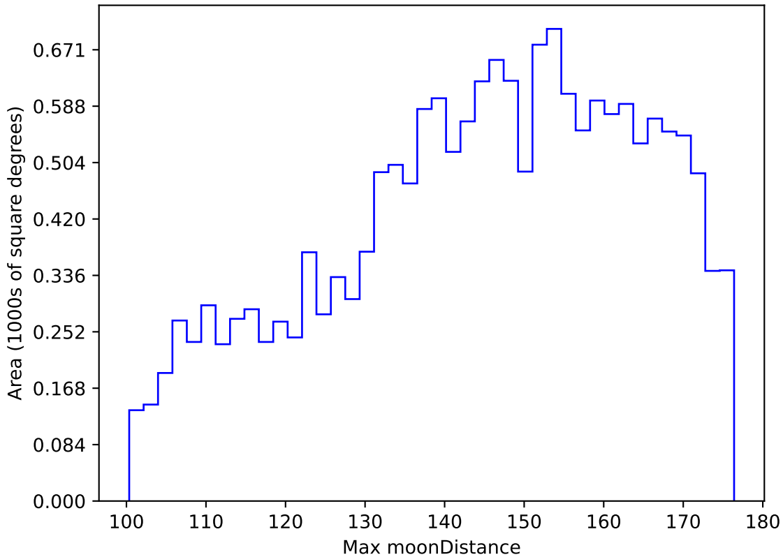
too_elab_r64_d2_ugrizy_v3.4_10yrs WFD y band: Max moonDistance
