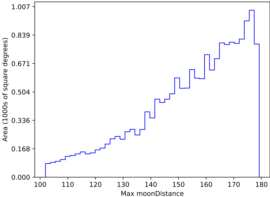
too_elab_r64_d2_ugrizy_v3.4_10yrs WFD u band: Max moonDistance
