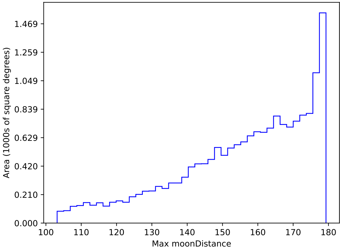
too_elab_r64_d2_ugrizy_v3.4_10yrs WFD r band: Max moonDistance
