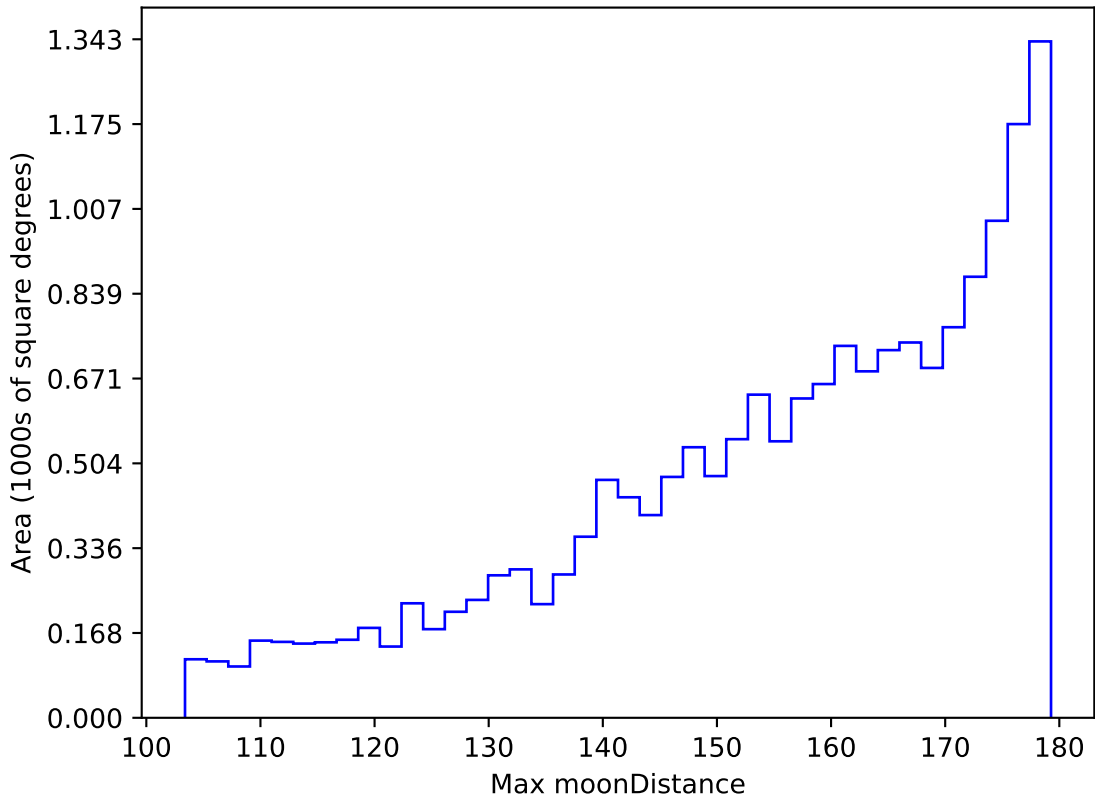
too_elab_r64_d2_ugrizy_v3.4_10yrs WFD i band: Max moonDistance
