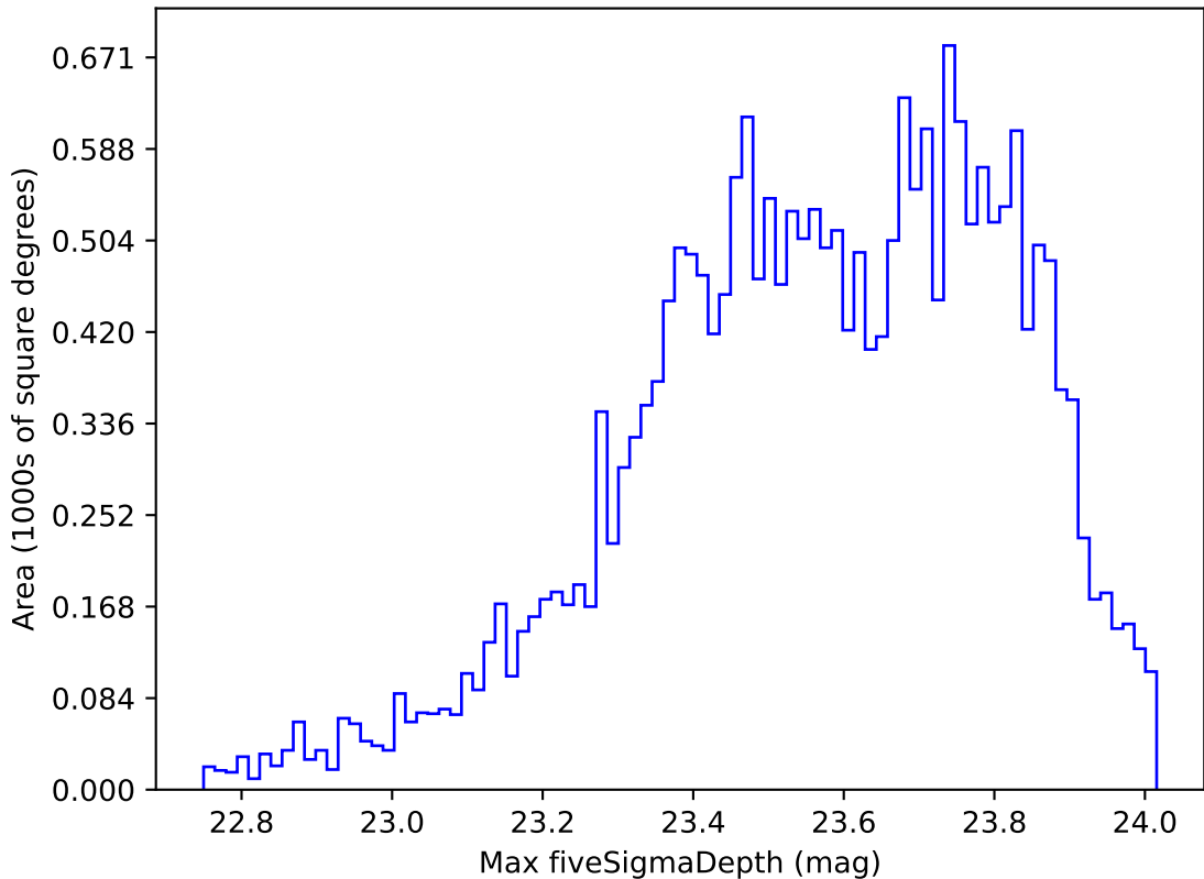
too_elab_r64_d2_ugrizy_v3.4_10yrs Yr 1 u band: Max fiveSigmaDepth
