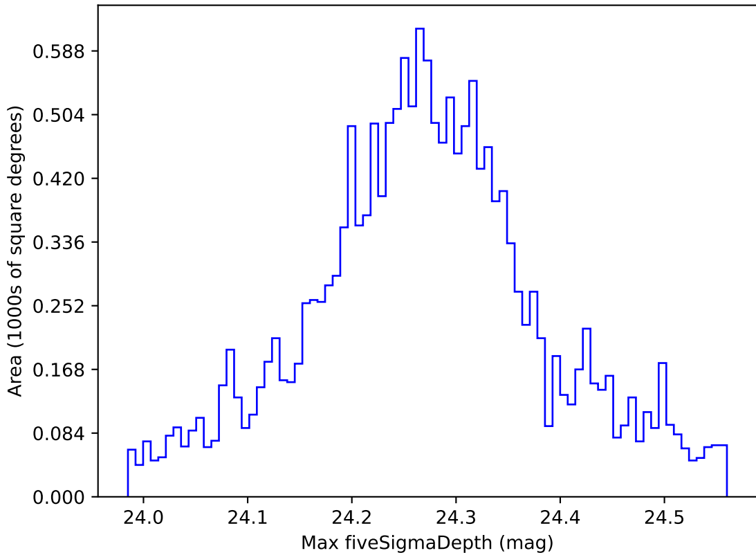
too_elab_r64_d2_ugrizy_v3.4_10yrs WFD i band: Max fiveSigmaDepth
