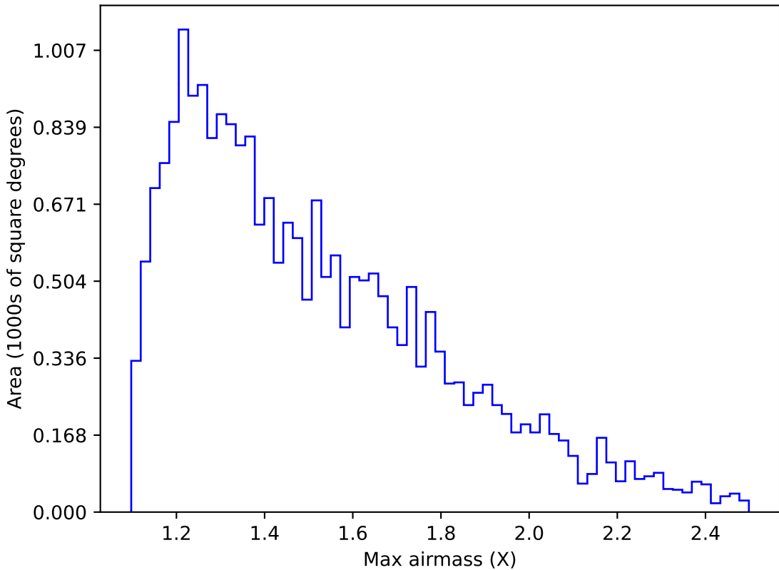
too_elab_r64_d2_ugrizy_v3.4_10yrs Yr 1 u band: Max airmass
