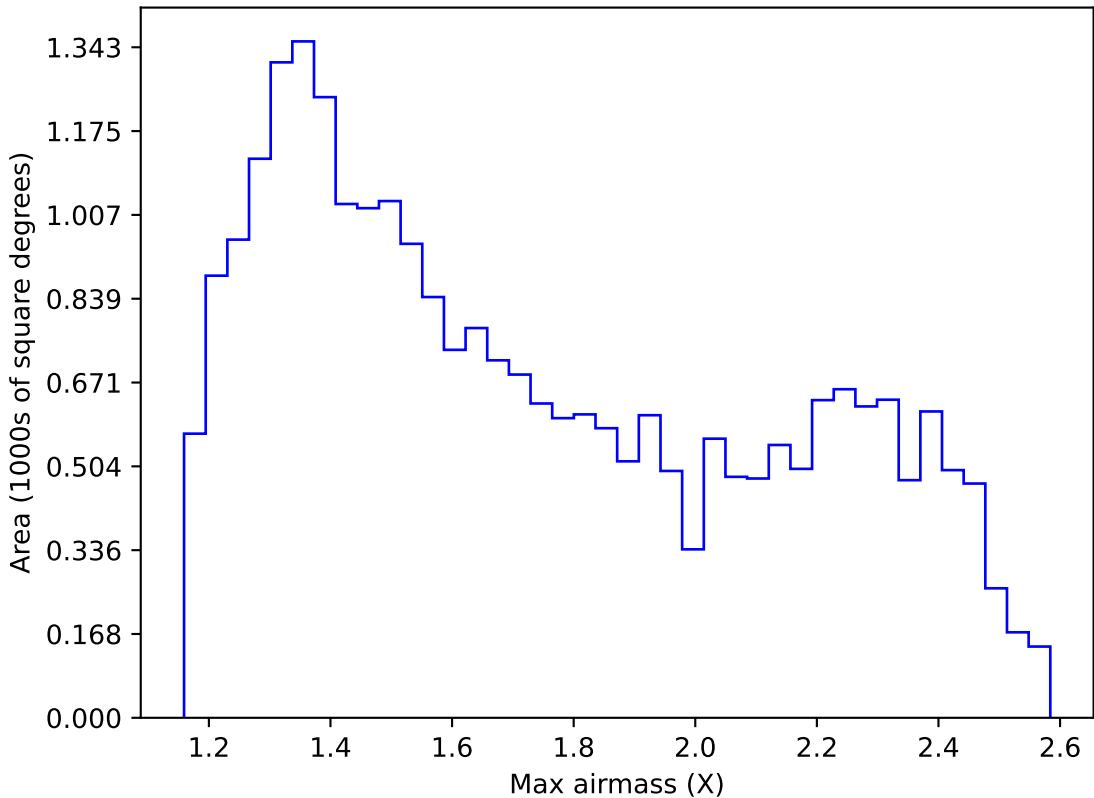
too_elab_r64_d2_ugrizy_v3.4_10yrs Yr 1 r band: Max airmass
