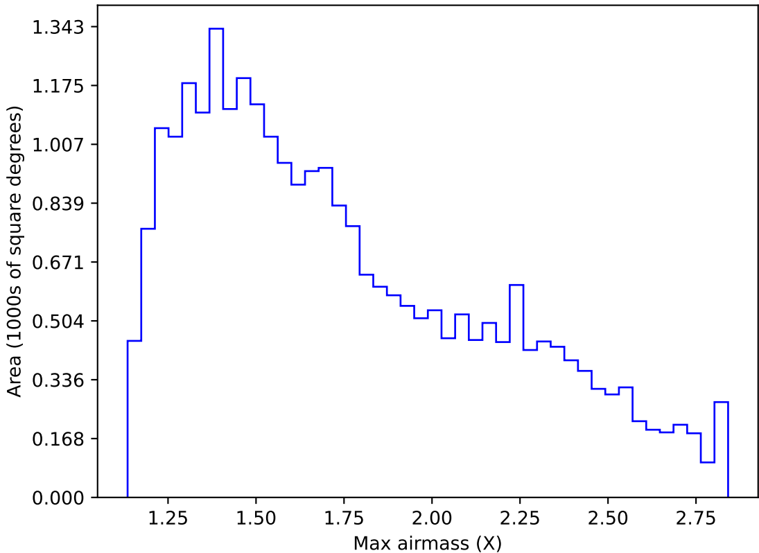
too_elab_r64_d2_ugrizy_v3.4_10yrs Yr 1 i band: Max airmass
