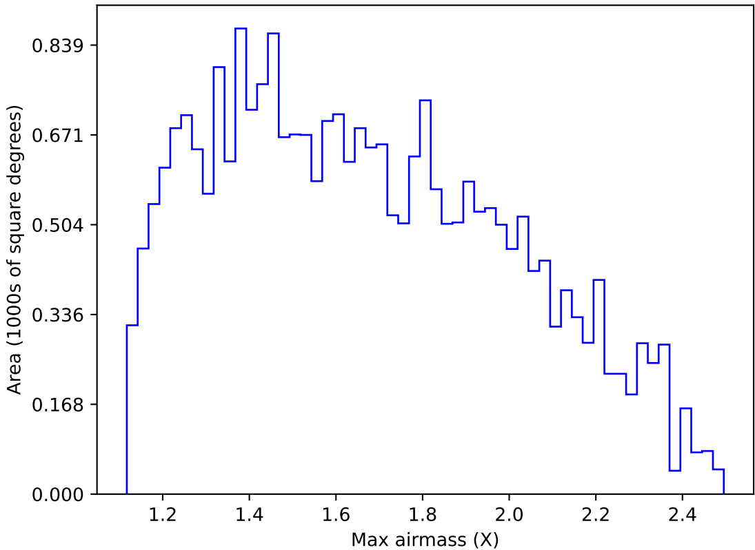
too_elab_r64_d2_ugrizy_v3.4_10yrs Yr 1 g band: Max airmass
