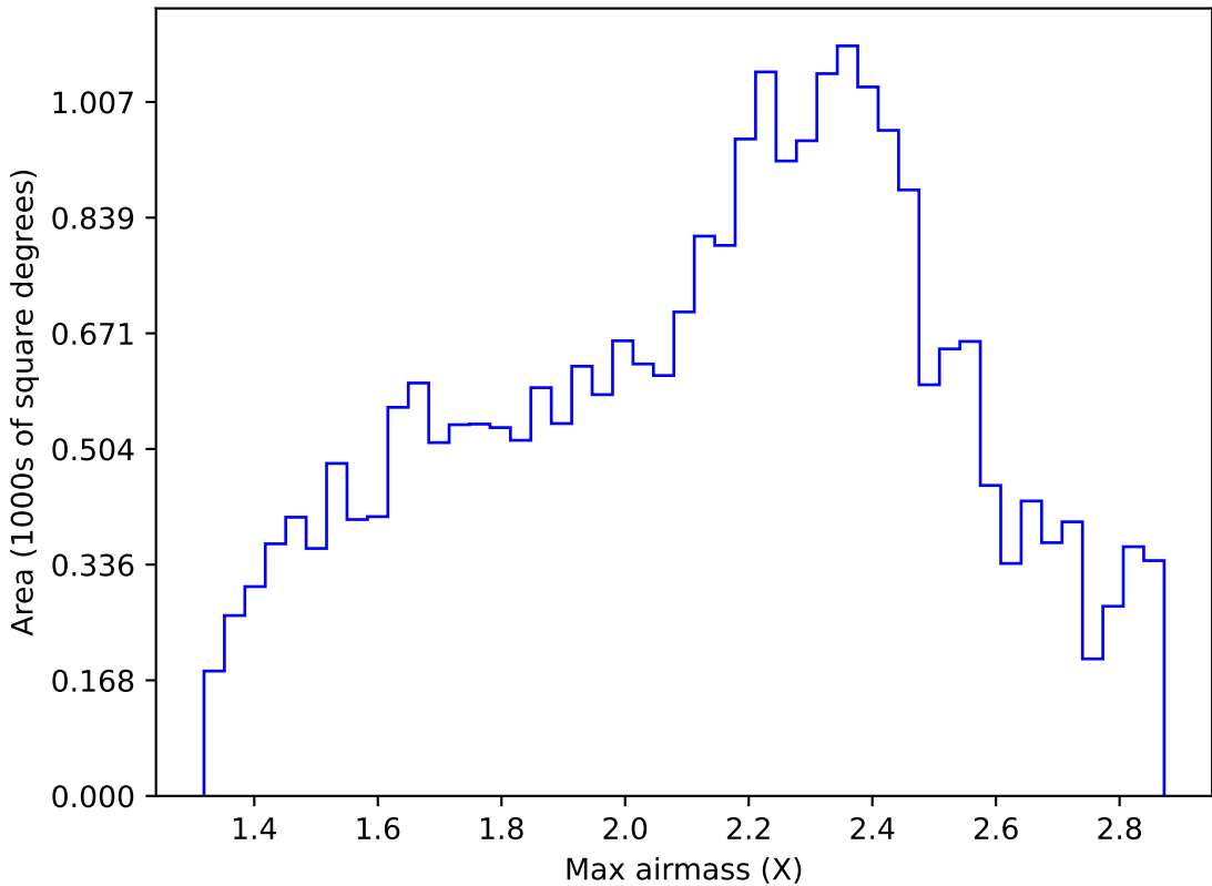
too_elab_r64_d2_ugrizy_v3.4_10yrs Yr 1 all bands: Max airmass
