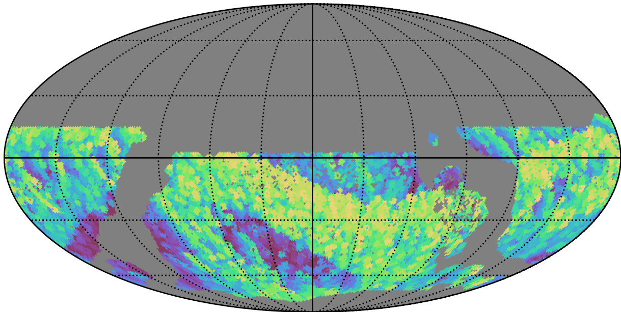
too_elab_r64_d2_ugrizy_v3.4_10yrs WFD z band: Max airmass
