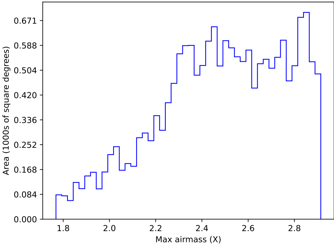
too_elab_r64_d2_ugrizy_v3.4_10yrs WFD z band: Max airmass
