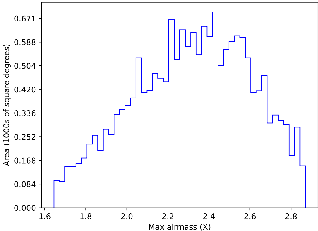
too_elab_r64_d2_ugrizy_v3.4_10yrs WFD y band: Max airmass
