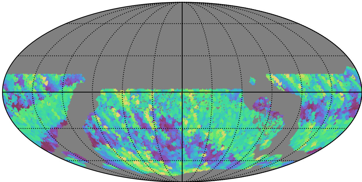
too_elab_r64_d2_ugrizy_v3.4_10yrs WFD r band: Max airmass
