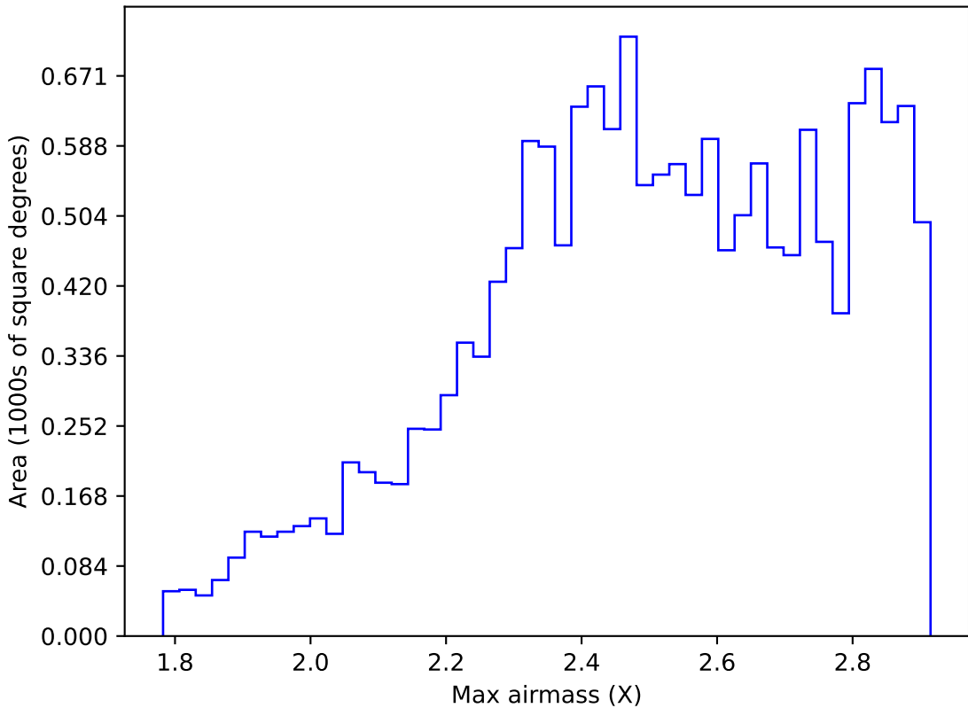
too_elab_r64_d2_ugrizy_v3.4_10yrs WFD i band: Max airmass
