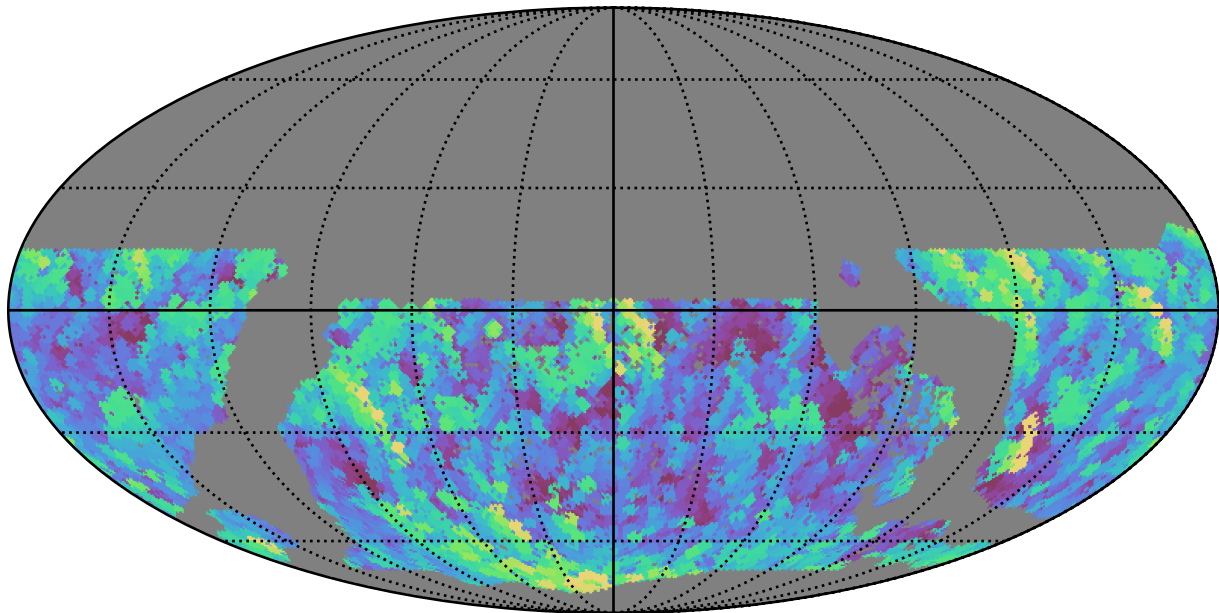
too_elab_r64_d2_ugrizy_v3.4_10yrs WFD g band: Max airmass
