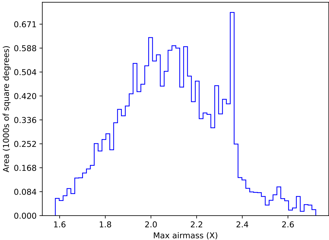
too_elab_r64_d2_ugrizy_v3.4_10yrs WFD g band: Max airmass
