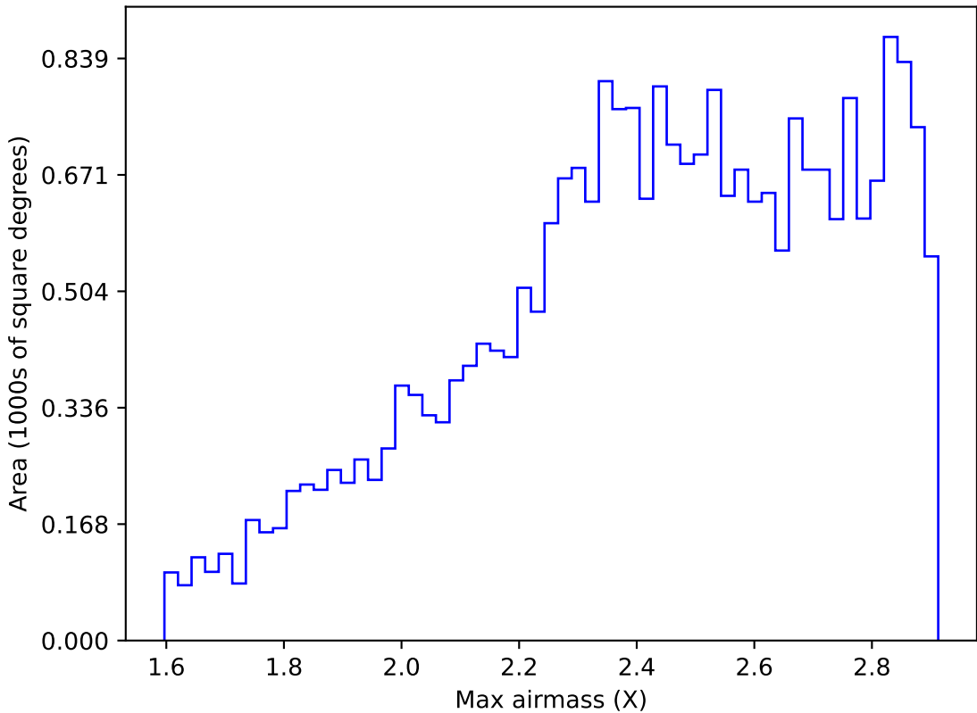
too_elab_r64_d2_ugrizy_v3.4_10yrs All sky z band: Max airmass
