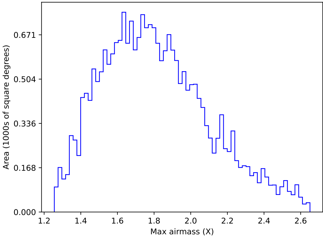
too_elab_r64_d2_ugrizy_v3.4_10yrs All sky u band: Max airmass
