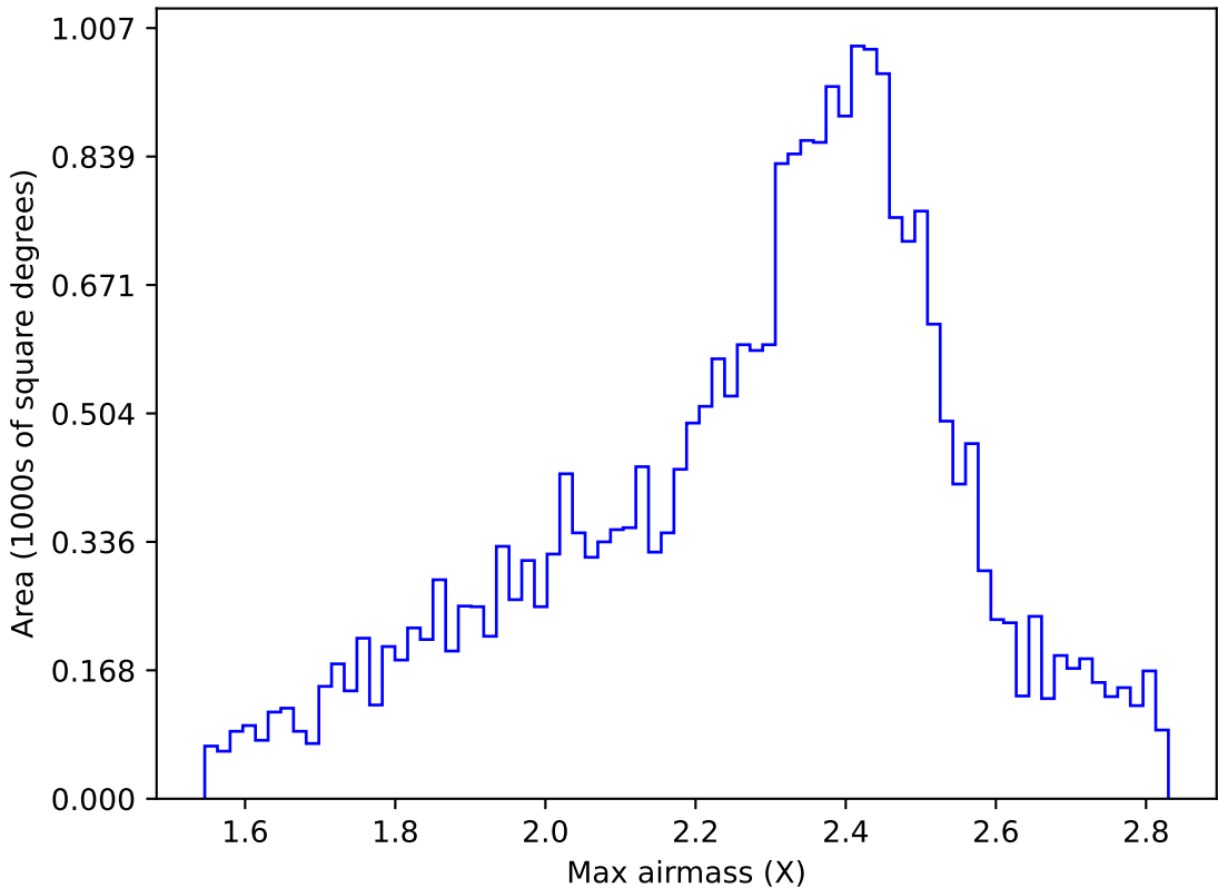
too_elab_r64_d2_ugrizy_v3.4_10yrs All sky r band: Max airmass
