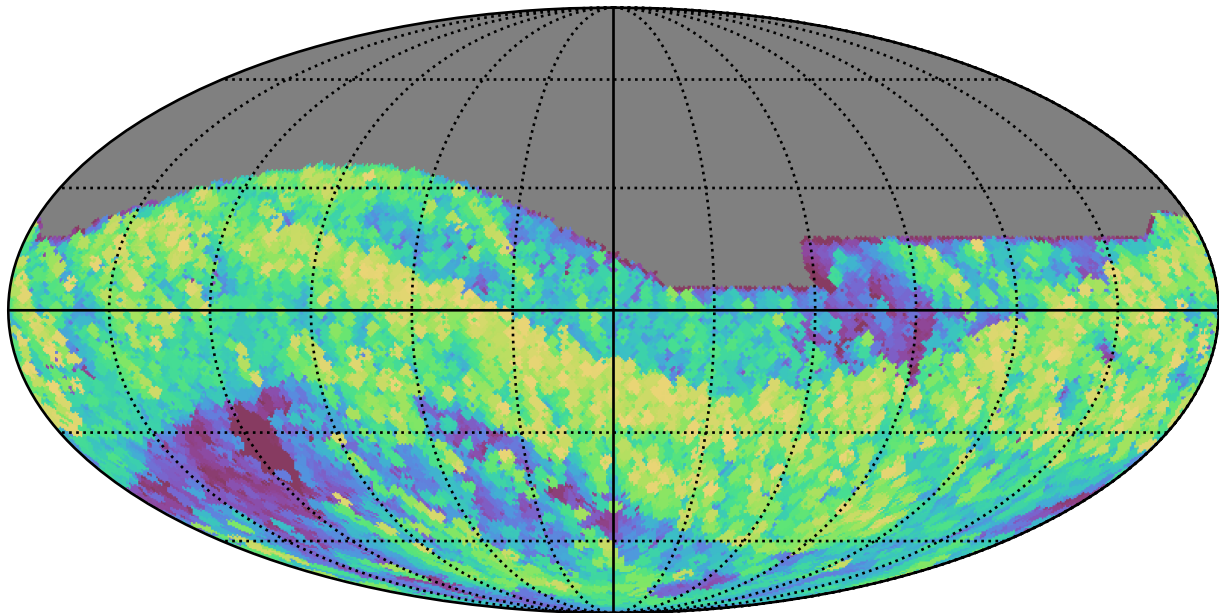
too_elab_r64_d2_ugrizy_v3.4_10yrs All sky i band: Max airmass
