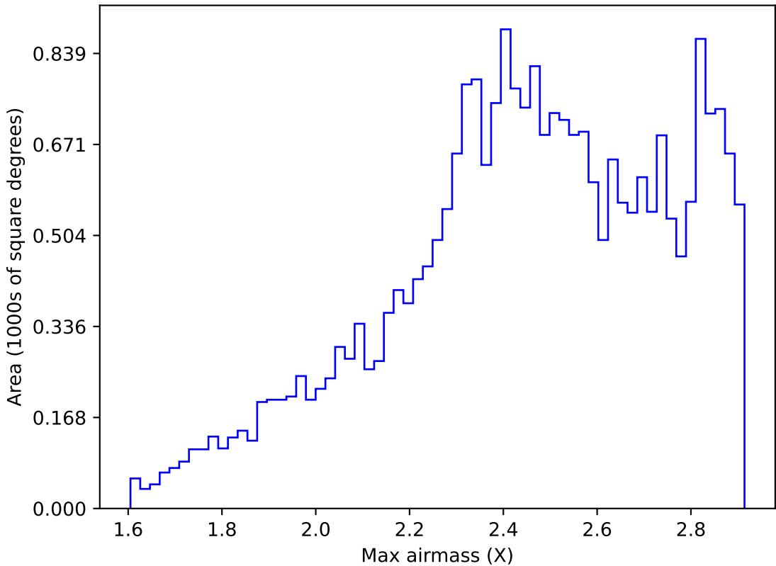
too_elab_r64_d2_ugrizy_v3.4_10yrs All sky i band: Max airmass
