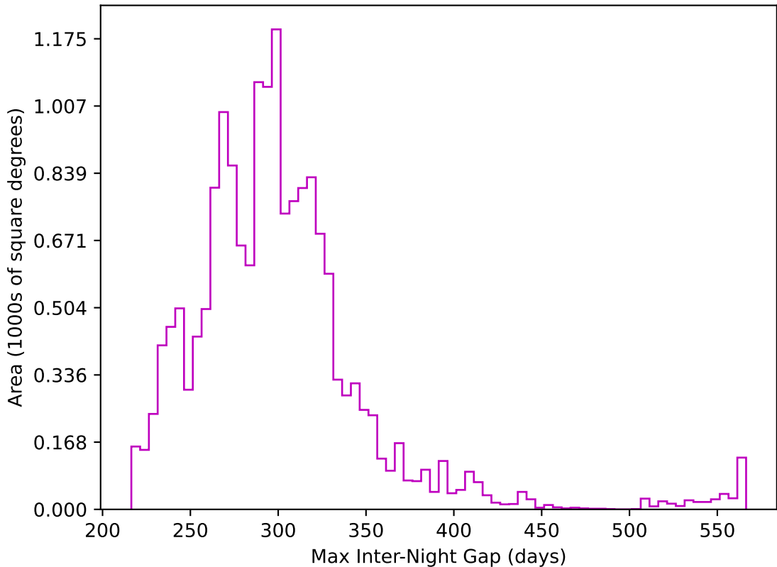
too_elab_r64_d2_ugrizy_v3.4_10yrs WFD z band: Max Inter-Night Gap
