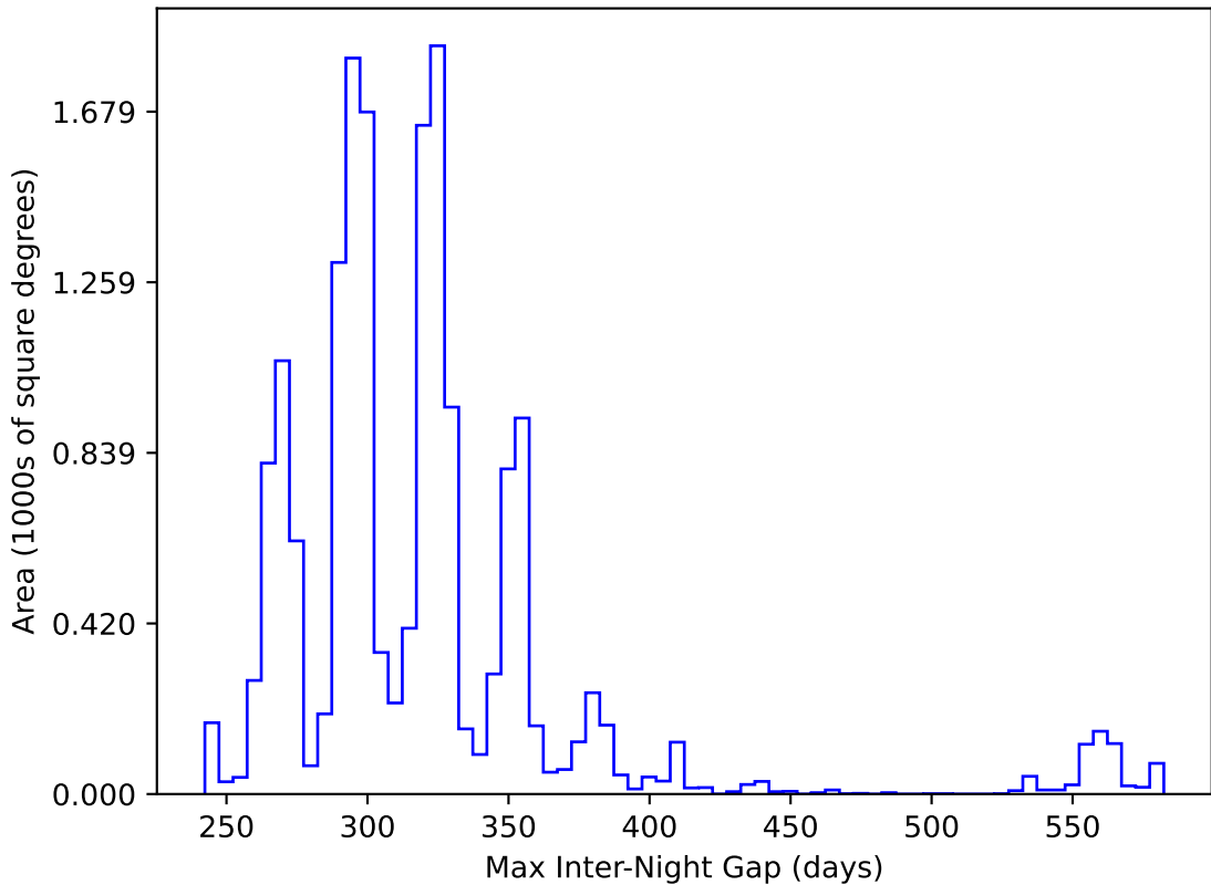
too_elab_r64_d2_ugrizy_v3.4_10yrs WFD y band: Max Inter-Night Gap
