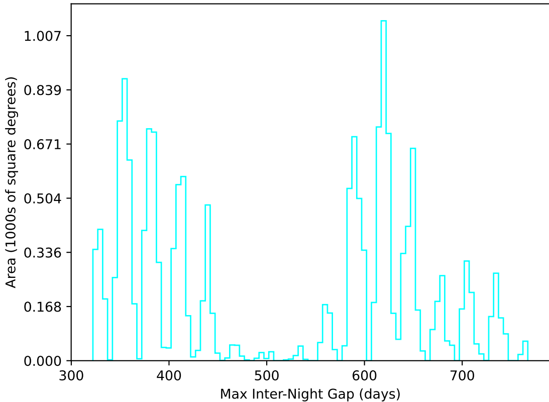
too_elab_r64_d2_ugrizyv3.4_10yrs WFD u band: Max Inter-Night Gap
