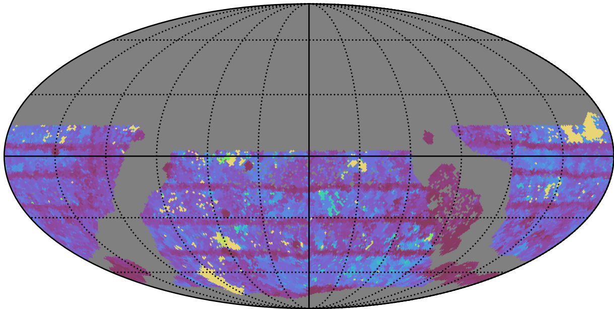
too_elab_r64_d2_ugrizy_v3.4_10yrs WFD r band: Max Inter-Night Gap
