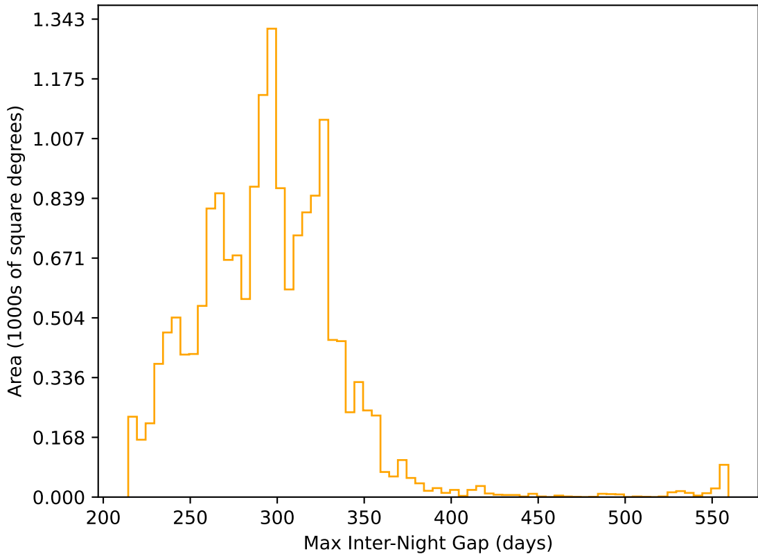
too_elab_r64_d2_ugrizy_v3.4_10yrs WFD r band: Max Inter-Night Gap
