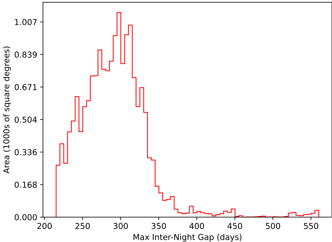
too_elab_r64_d2_ugrizy_v3.4_10yrs WFD i band: Max Inter-Night Gap
