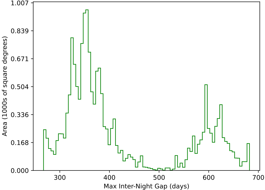
too_elab_r64_d2_ugrizy_v3.4_10yrs WFD g band: Max Inter-Night Gap
