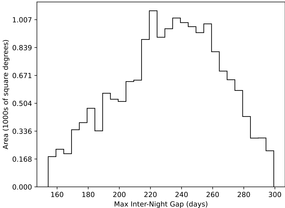
too_elab_r64_d2_ugrizy_v3.4_10yrs WFD all bands: Max Inter-Night Gap
