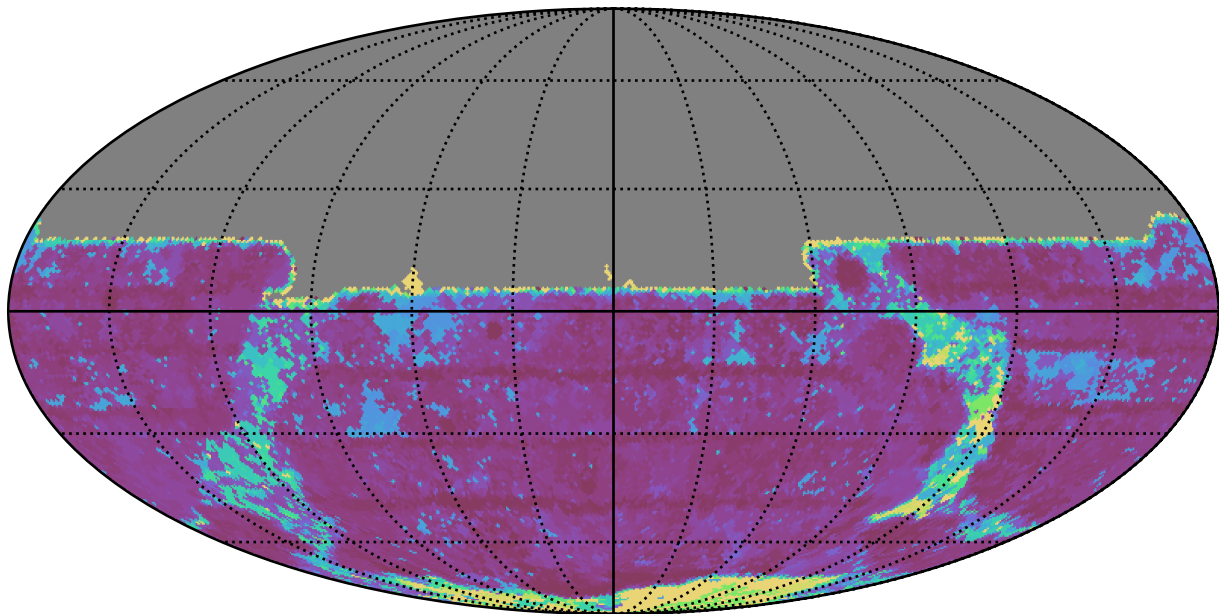
too_elab_r64_d2_ugrizy_v3.4_10yrs All sky y band: Max Inter-Night Gap
