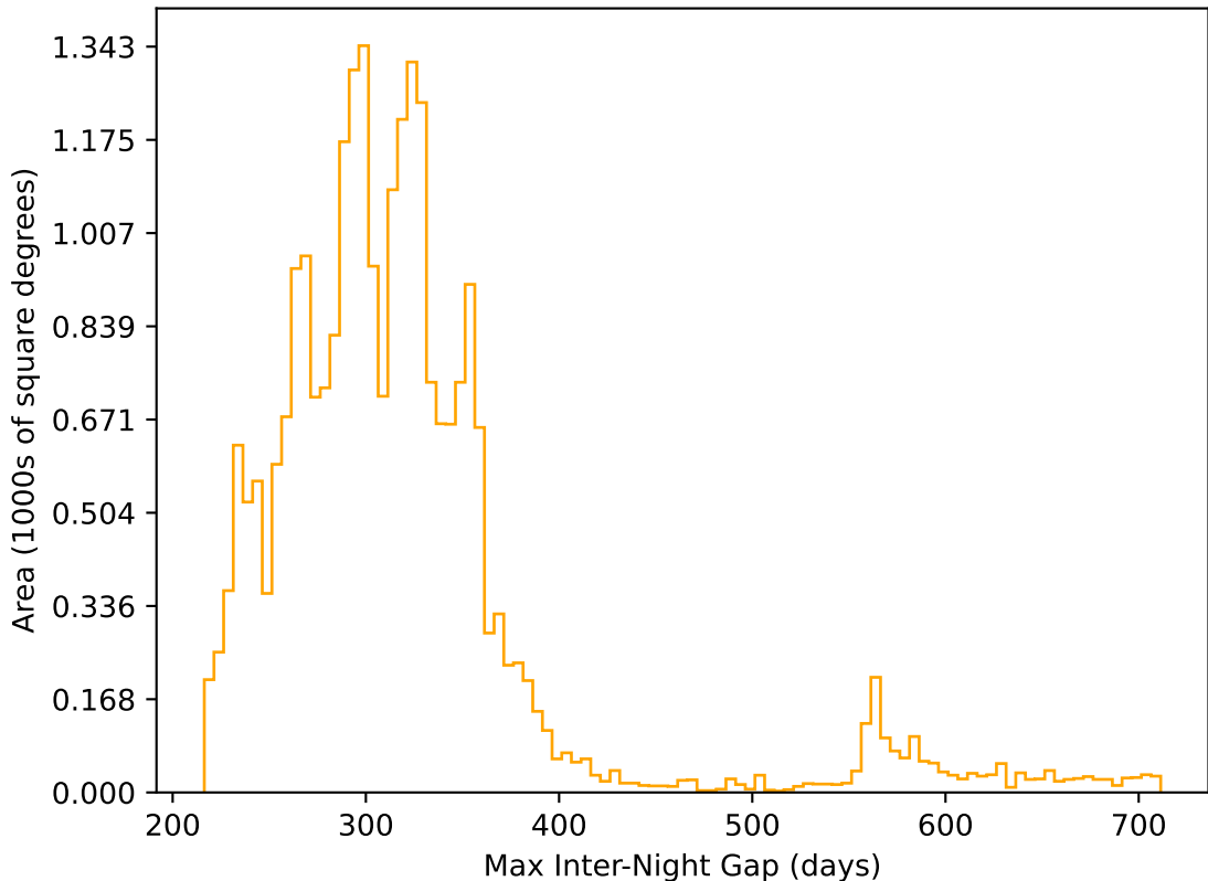
too_elab_r64_d2_ugrizy_v3.4_10yrs All sky r band: Max Inter-Night Gap
