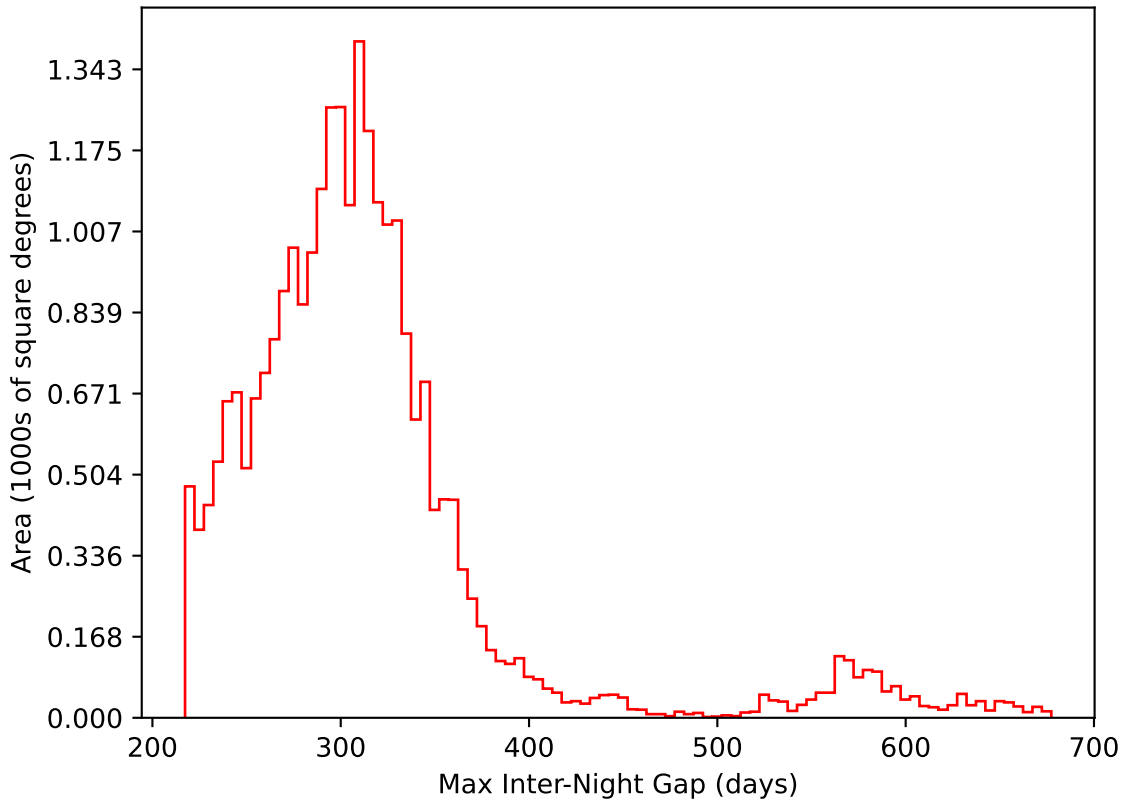
too_elab_r64_d2_ugrizy_v3.4_10yrs All sky i band: Max Inter-Night Gap
