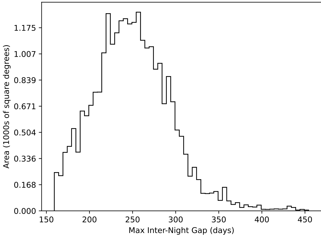
too_elab_r64_d2_ugrizy_v3.4_10yrs All sky all bands: Max Inter-Night Gap
